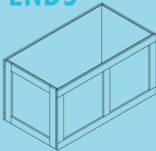
Plywood panels 1x4 cleats
